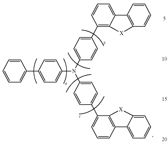
Chemical Formula 2
