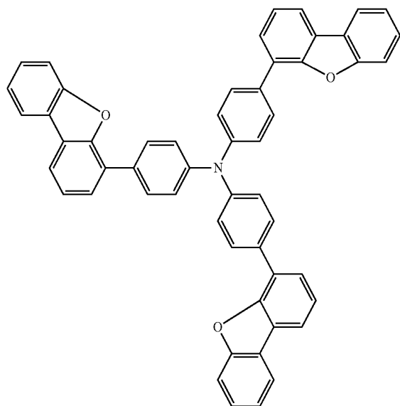
Chemical Formula 1-1
