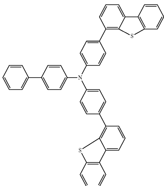
Chemical Formula 2-5
