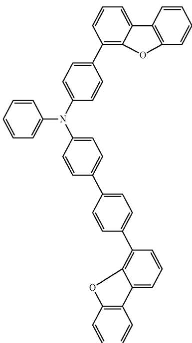
Chemical Formula 2-4
