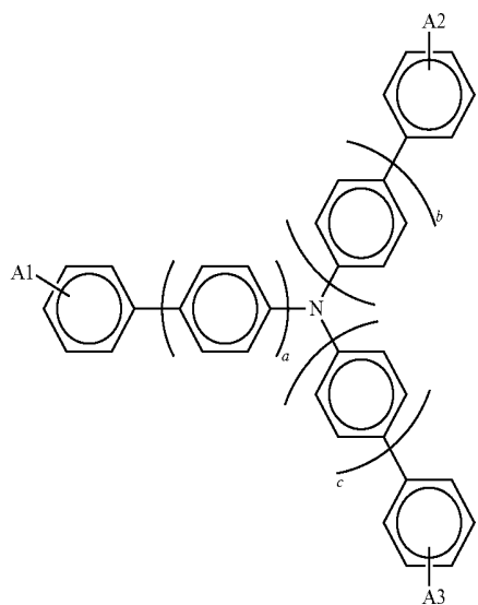
Chemical Formula 1
