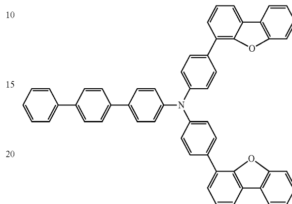
Chemical Formula 2-2
