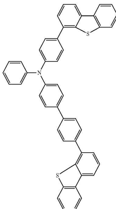
Chemical Formula 2-6
