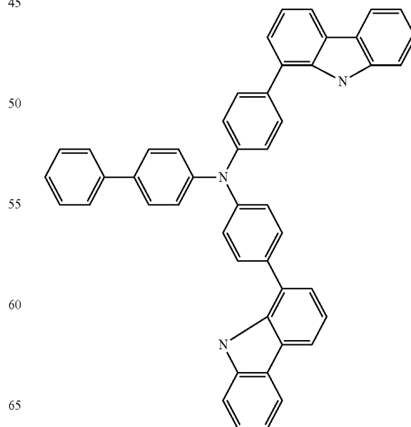
Chemical Formula 2-3
