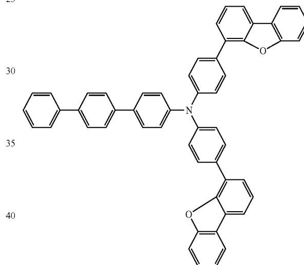
Chemical Formula 2-3
