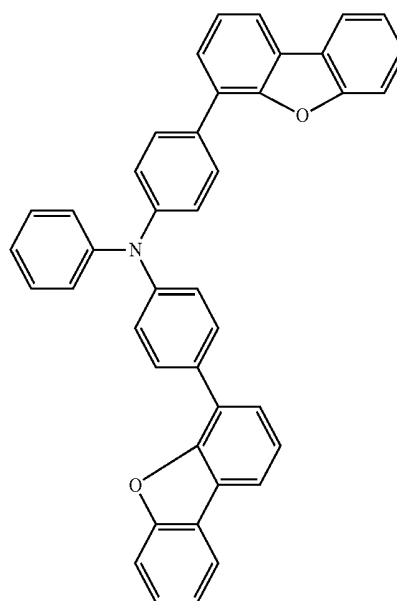
Chemical Formula 1-2
